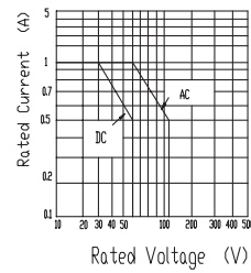
Contact Switching Capacity
